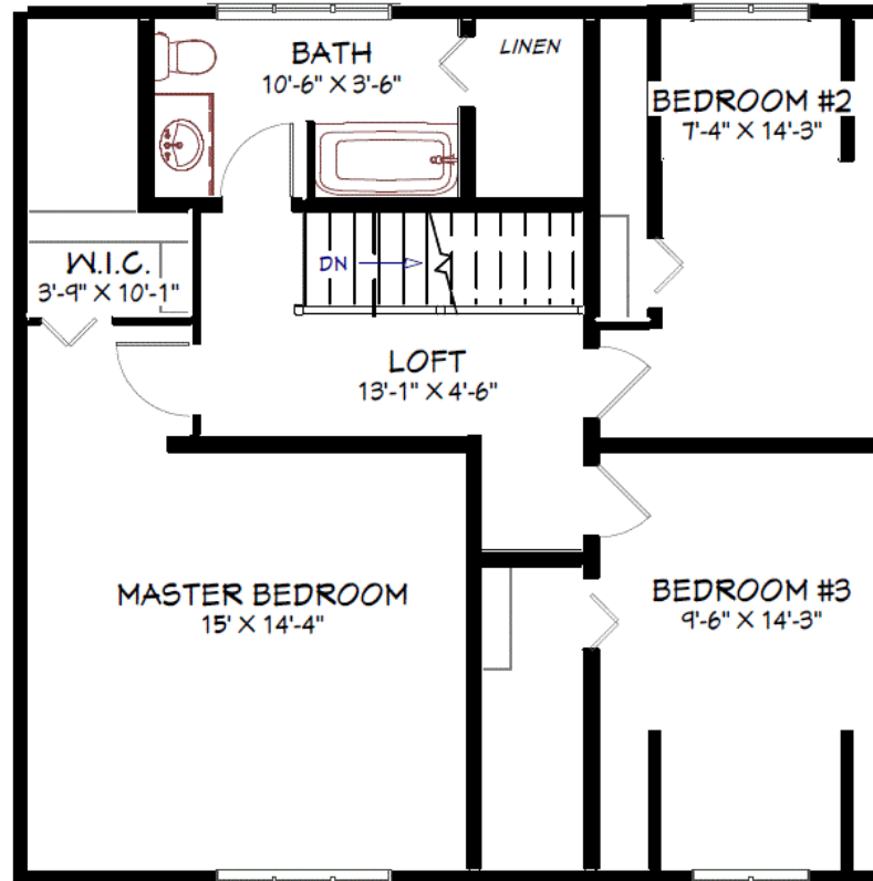
UPPER FLOOR
