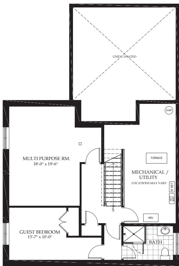
LOWER LEVEL FINISHED AREA, 610 SQ. FT.
